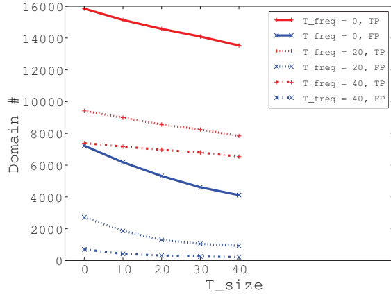
Figure 9: The number of TPs and FPs in the detection result, varying the minimum domain frequency and minimum segment size thresholds.
