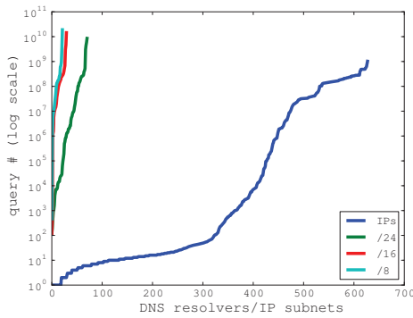
Figure 3: Outgoing DNS queries generated by various resolvers, sorted by volume and aggregated by IP addresses, and /24, /16 and /8 subnets.
